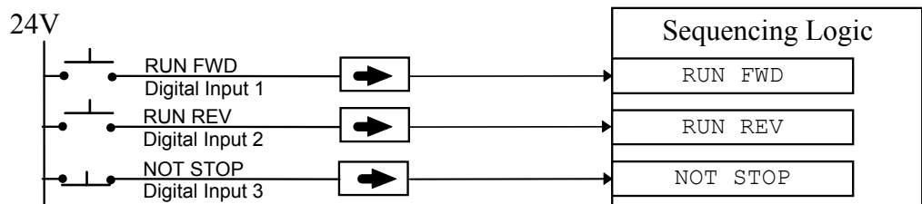
Figure Chapter 4 -14 Wiring for Three Wire Logic Starting
