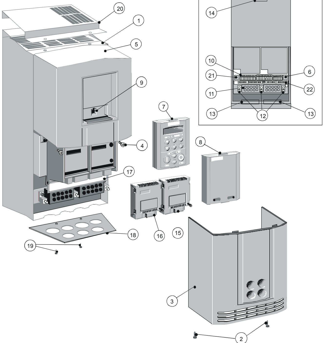
Figure Chapter 2 -3 690+ AC Drive, Frame D 15 - 22kW
