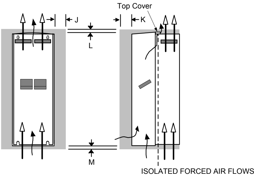
Figure Chapter 3 -11 Air Clearance for a Wall-Mount Product/Application
