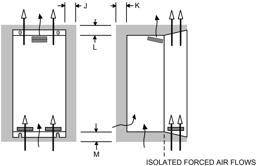
Figure Chapter 3 -7 Air Clearance for a Cubicle-Mount Product/Application
