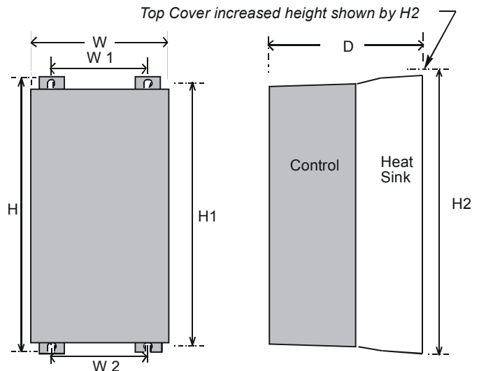
Figure Chapter 3 -1 Mechanical Dimensions for 690+ Series
