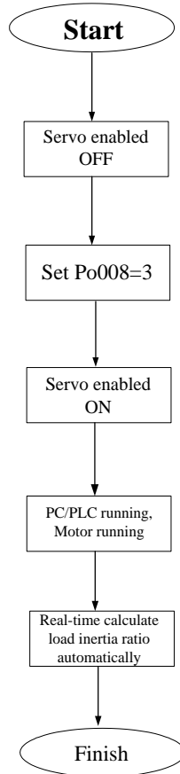
Fig 7.2.2 Online rotational inertia setting flow chart
