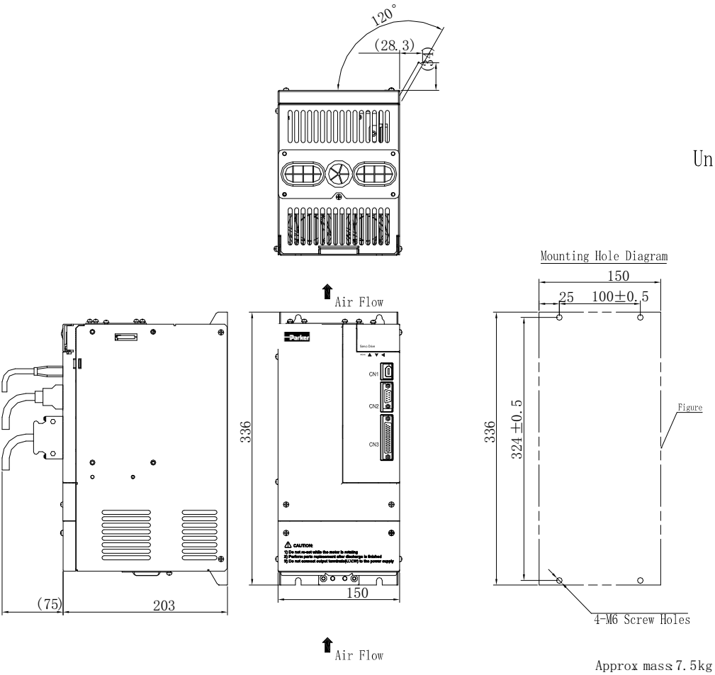
Fig 3.1.6 Servo drive structure 4
