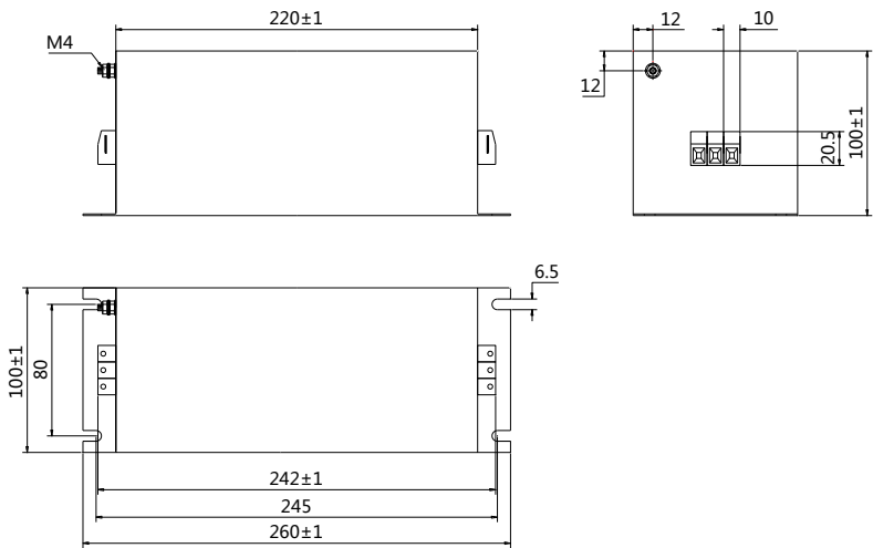
Fig 2.4.4 FT330F series
