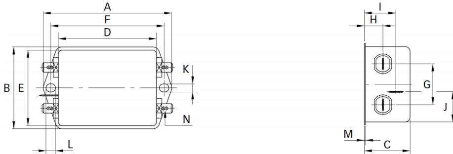
Fig 2.4.5 FN2090 series
