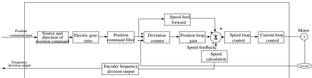
Fig 6.4.1 Position pulse mode block diagram
