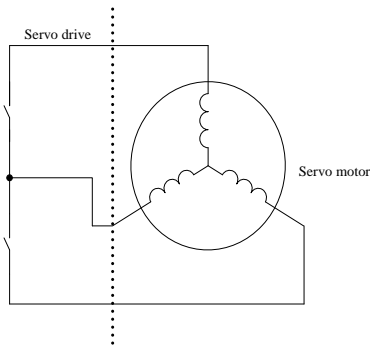
Fig 6-1-9 Dynamic braking
