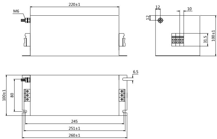
Fig 2.4.3 FT330F series
