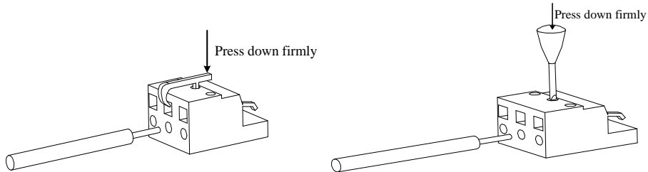
Fig 4.1.3 Connection procedure
